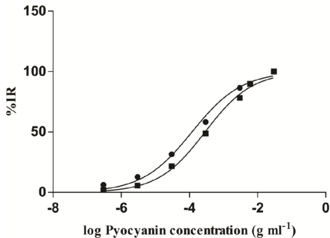
Figure 4. Logarithmic scales of C_{11} and E_8 pyocyanin concentrations against %IR. IC_{50} of C_{11} pyocyanin calculated by the GraphPad Prism software showed a greater result than E_8 with significant difference ( P < 0.0001 )
