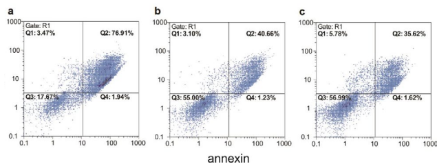
Figure 5. Dot plot results of annexin/PI staining of Panc-1 cells treated by (a) 1.5 \text{ mg.ml}^{-1} (b) 300 \text{ µg.ml}^{-1} (c) 150 \text{ µg.ml}^{-1} of C_{11} pyocyanin that induced apoptosis and/or necrosis in 82.33, 45, and 43.01% of Panc-1 cells, respectively. Q_1 : necrotic cells, Q_2 : apoptotic and necrotic cells, Q_3 : viable cells, Q_4 : apoptotic cells
