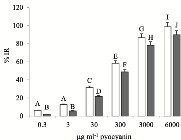
Figure 3. T-test analysis of the comparison between C 11 and E 8 pyocyanin cytotoxicity. C 11 pyocyanin showed higher cytotoxicity than E 8 with significant differences in all treated groups. Several letters represent in- and between-group significant differences ( P < 0.05 )
