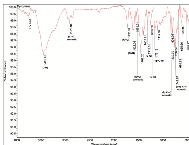
Figure 2. FT-IR spectrum of C 11 pyocyanin (C 13 H 10 N 2 O)
