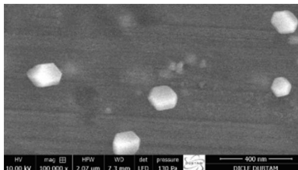
Figure 3. SEM images of the GP-SLN formulation showing cubical shaped nanoparticles SEM: Scanning electron microscopy; GP-SLN: Gabapentin loaded solid lipid nanoparticle formulation
