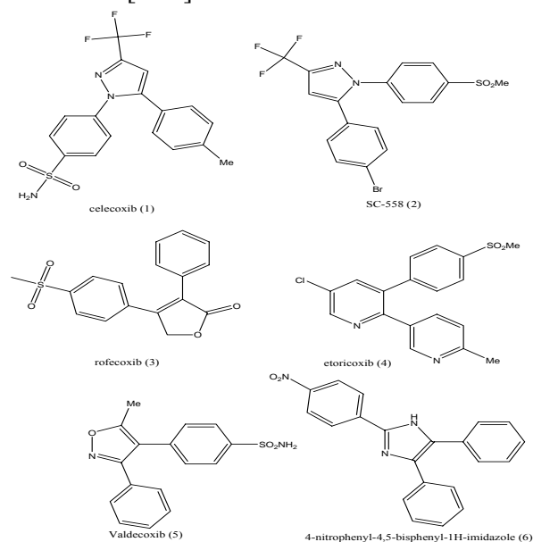
Figure 1. Representative examples of COX-2inhibitors.
