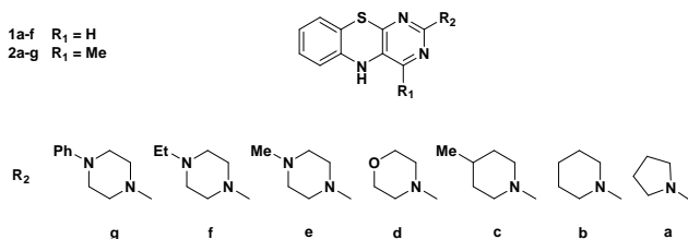
Scheme 1: chemical structure of compounds 1a-f and 2a-f
