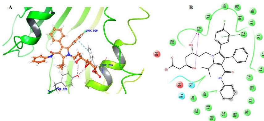
Figure 1. The molecular docking of atorvastatin against TLR2 protein (A) The binding mode of atorvastatin (brown) is depicted, and key residues are marked with grey sticks. (B) A log plot of atorvastatin is displayed in the active site of the TLR2 protein receptor TLR: Toll-like receptor
