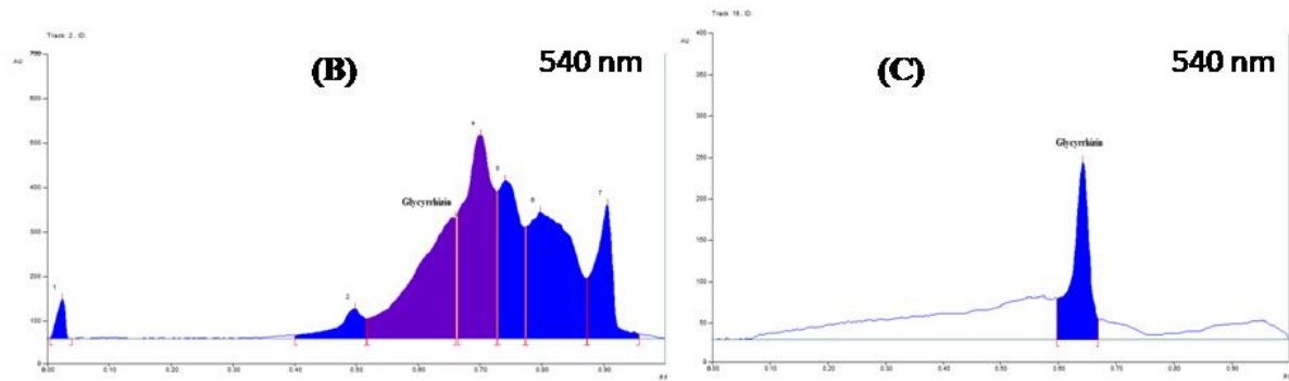
Supplementary Figure 1: HPTLC plate view and chromatograms of GGE at 540 nm. Panel (A) represents track of sample and standard and (B)-(C) show chromatograms of the sample and standard at 540 nm
