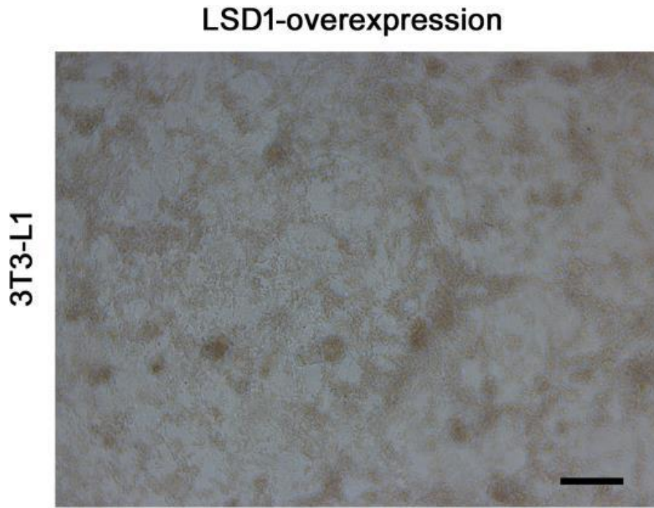
Figure S1. Morphology of 3T3-L1 infected with LSD1-overexpression lentivirus
