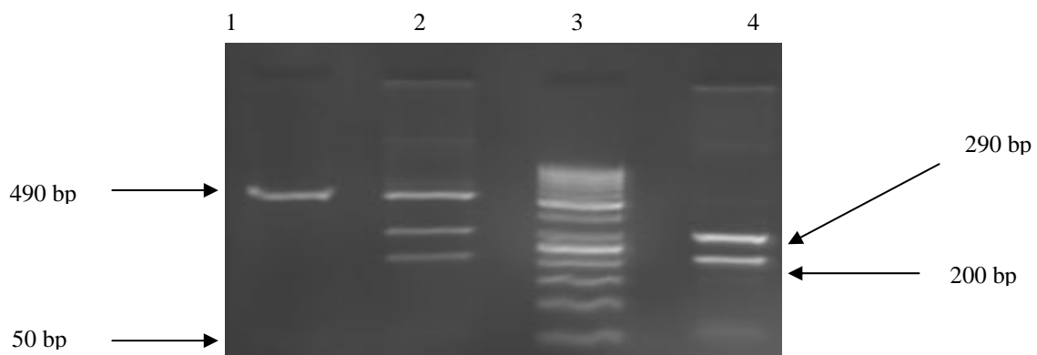
Figure 1. An ethidium bromide stained agarose gel showing PCR-RFLP analysis of exon 9 of the VDR gene. The gel illustrates Taq -1 digestion of the VDR exon 9 amplicon which contains a known Taq -1 RFLP. Lane 1: homozygous PCR product, which is not susceptible to Taq -1 digestion ( t/t ). Lane 2: heterozygous digestion ( T/t ). Lane 3: 50 bp ladder marker and lane 4: homozygous digestion ( T/T ).
