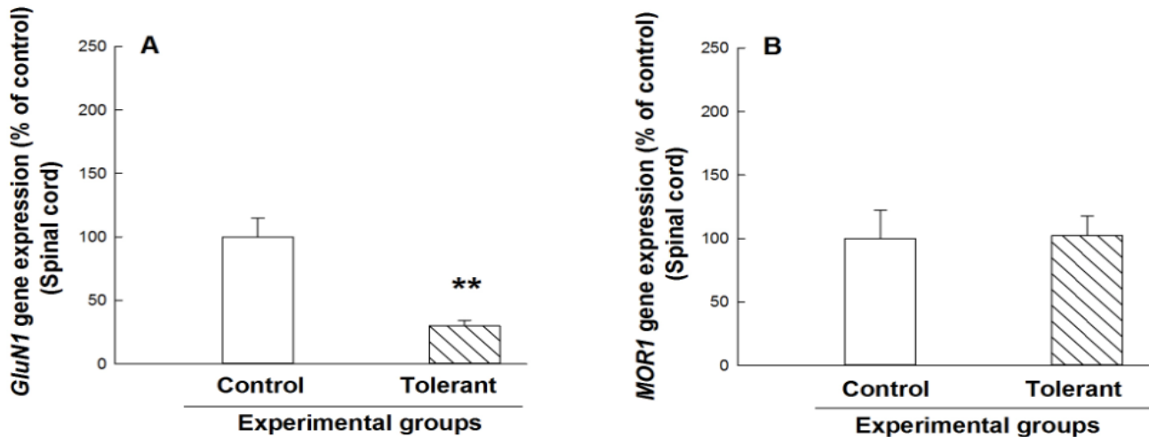
Figure 4. Relative gene expression of the GluN1 (panel A) and the MOR1 (panel B) in the lumbar spinal cord in control and tolerant groups. Each bar represents mean \pm SEM of quantified data related to the expression of the respective genes in each group. ** P < 0.01 compared to the saline-treated control group
