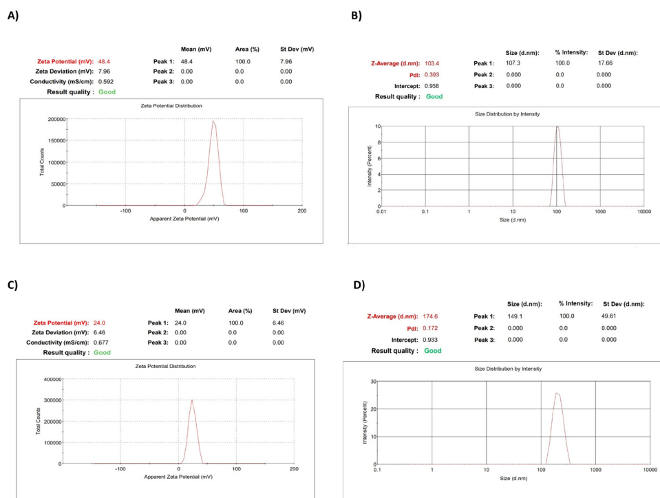
Figure 1. Nanoparticles characterization
