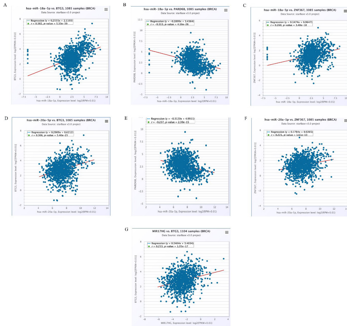
Figure 6. Expression relationship scatter plot between miRNAs and their targets based on the starBase web platform. Within the PanCancer section of starBase, the analysis identifies significant associations between miR-18a and its mRNA targets in cases of invasive breast carcinoma (A, B, C). Furthermore, analogous relationships have been documented for mir-20a-5p and its mRNA targets (D, E, F), in addition to the interaction between MIR17HG and BTG3 (G) (Created using starBase, Microsoft PowerPoint)
