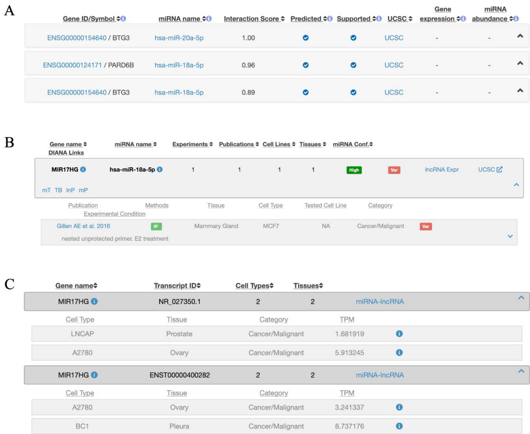
Figure 4. Assessment of investigated miRNA-lncRNA-mRNA interactions based on some databases (A) Evaluation of miRNA-mRNA interactions using the microT web server (20): The miRNA-mRNA relationships identified in our analysis were evaluated with microT, which provides results from other studies. (B) Evaluation of miRNA-lncRNA interactions using the LncBase web platform (21, 22). This platform indicates whether any studies have identified a miRNA target for the specified lncRNA. It indicates that miR-18a has been reported as a target for MIR17HG in a study related to cancerous mammary glands, showing a strong correlation. (C) According to LncBase, MIR17HG has been implicated in cancers of the prostate, ovary, and pleura (Created using microT web server, LncBase web platform, Microsoft PowerPoint).
